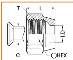
減壓螺帽 Reducing Nut
