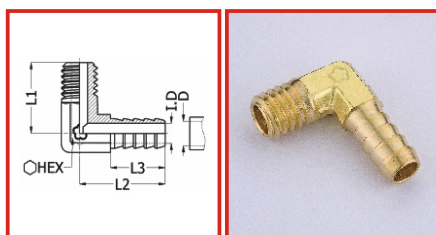
惠氏牙插心彎頭 Whitworth male Hose-Barb Elbow
