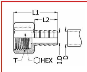
內牙插心接頭 Female Hose-Barb Connector
