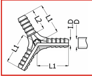
Y 型插心三通 Y-Type Union Hose-Barb
